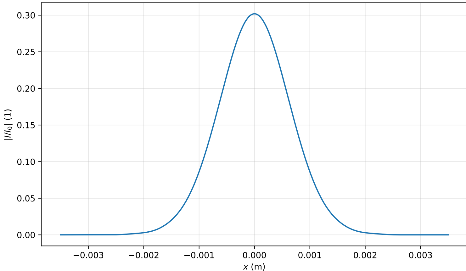
Intensity profile I(x, y = 0, z = 3.503m)/I_0 , P_{in}=0.2P_{cr} , artificial time
